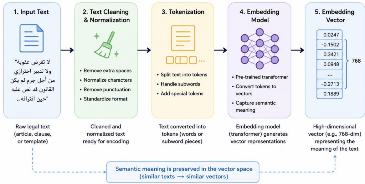
Figure 6 :Text-to-Embedding Process
